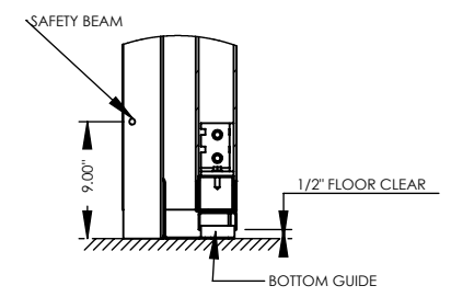
DETAIL SECTION "A-A"
